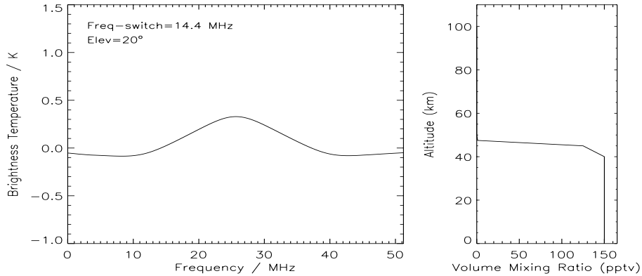
Figure 5. Simulation with MOLIERE CSO spectrum using a "truncated" HCN volume mixing ratio profile shown on the right of the picture. This profile, which indicates no HCN above 45 km, was used in the simulation, which indicates no HCN above 45 km, we obtain a spectrum close (in intensity) to the one measured on Nov. 19, 1999 from 05:00 to 06:00 at CSO (see Figure 3).
