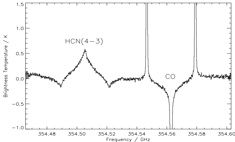
Figure 2. The HCN(4-3) line at 354.51 GHz (left part of the spectrum) observed at JCMT a day without strong meteor shower activity (25 th March, 1998). The frequency switch throw was 16.2 MHz and the integration time 1.5 h. The CO line on the right side of the spectrum comes from the image band of the radiometer and is therefore negative. The mesospheric CO line illustrates the expected width for high ( > 70 km) altitude molecules.
