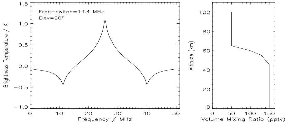
Figure 4. Simulation with MOLIERE of a CSO spectrum and the associated reference HCN volume mixing ratio profile (1pptv = 10^{-12} ) used for the computation (here the same profile than the "MOLIERE priori" HCN profile plotted in Figure 1).
