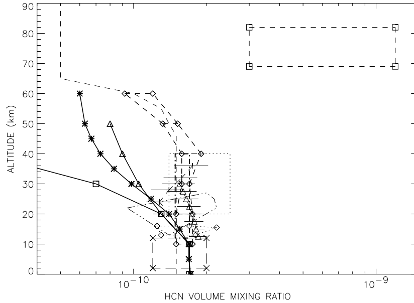
Figure 1. HCN in the atmosphere: models (thick black lines) and observations (others). Observations cover southern mid-latitudes (triangle; Zander et al. , 1988) to northern high latitudes (-.-.; Spreng and Arnold, 1994), using mass spectrometry (- - - with square; Kopp, 1990), infra-red (+++; Abbas et al. , 1987), and millimeter-wave techniques (- - - with diamond; Jaramillo et al. , 1988), with ground-, aircraft-based, balloon-, rocket-, and space-borne sensors. Photochemical models (thick black lines) are from Brasseur et al. (1985, with triangle for a photodissociation rate J_{\text{HCN}}=0 , and with square for J_{\text{HCN}}=J_{\text{HCL}} ) and Cicerone and Zellner (1983, with asterisk). A deficit in modeled HCN appears in the middle atmosphere, although tropospheric amounts agree reasonably well. Note the discrepancy between the photochemical models and the Kopp data around 75 km (dashed rectangle in the upper right corner of the plot). The other data are from Coffey et al. (-.-.; 1981), Carli et al. (...; 1982), Rinsland et al. (x-x; 1982), and Schneider et al. (... with diamond; 1997). The dashed line without symbol represents the a priori HCN profile used in radiative transfer calculations.
